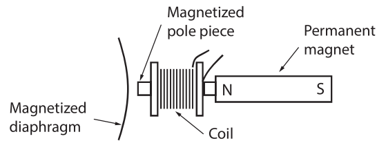
FIGURE 2.1 Diagram (side view) of Channing's 1877 handle telephone.
