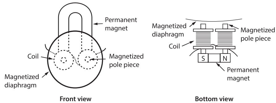
FIGURE 2.7 Diagrams of Bell's 1877 wall-mounted box telephone.
