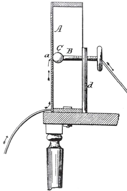
FIGURE 4.1 Drawing of a pressure-sensitive resistance transmitter from Berliner's patent. (Reprinted from Berliner 1891.)
