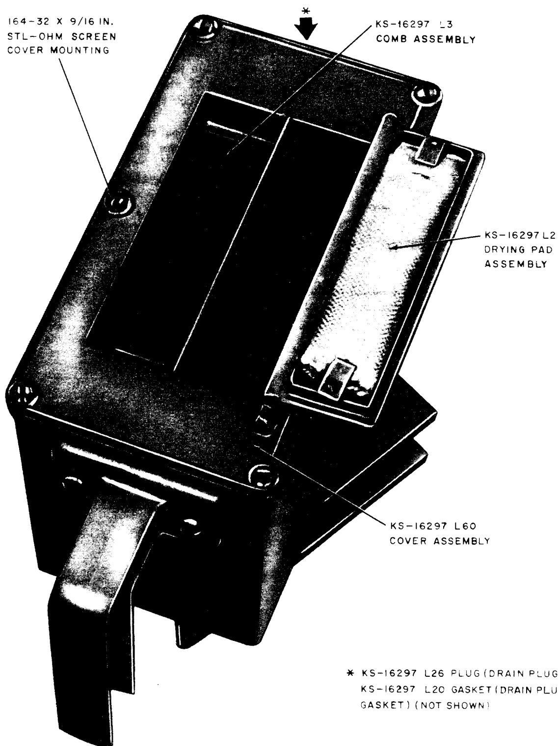
Fig. 14—Replaceable Parts of KS-16297 L70 Flushing Unit
