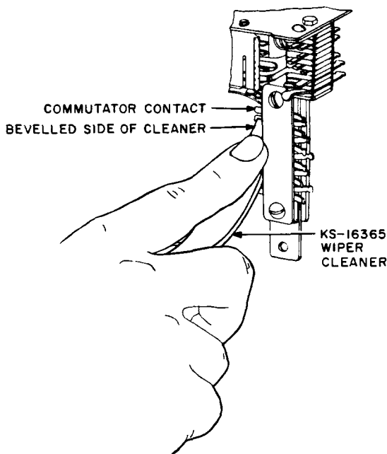
Fig. 3—Method of Nonabrasively Cleaning Commutator Contacts
