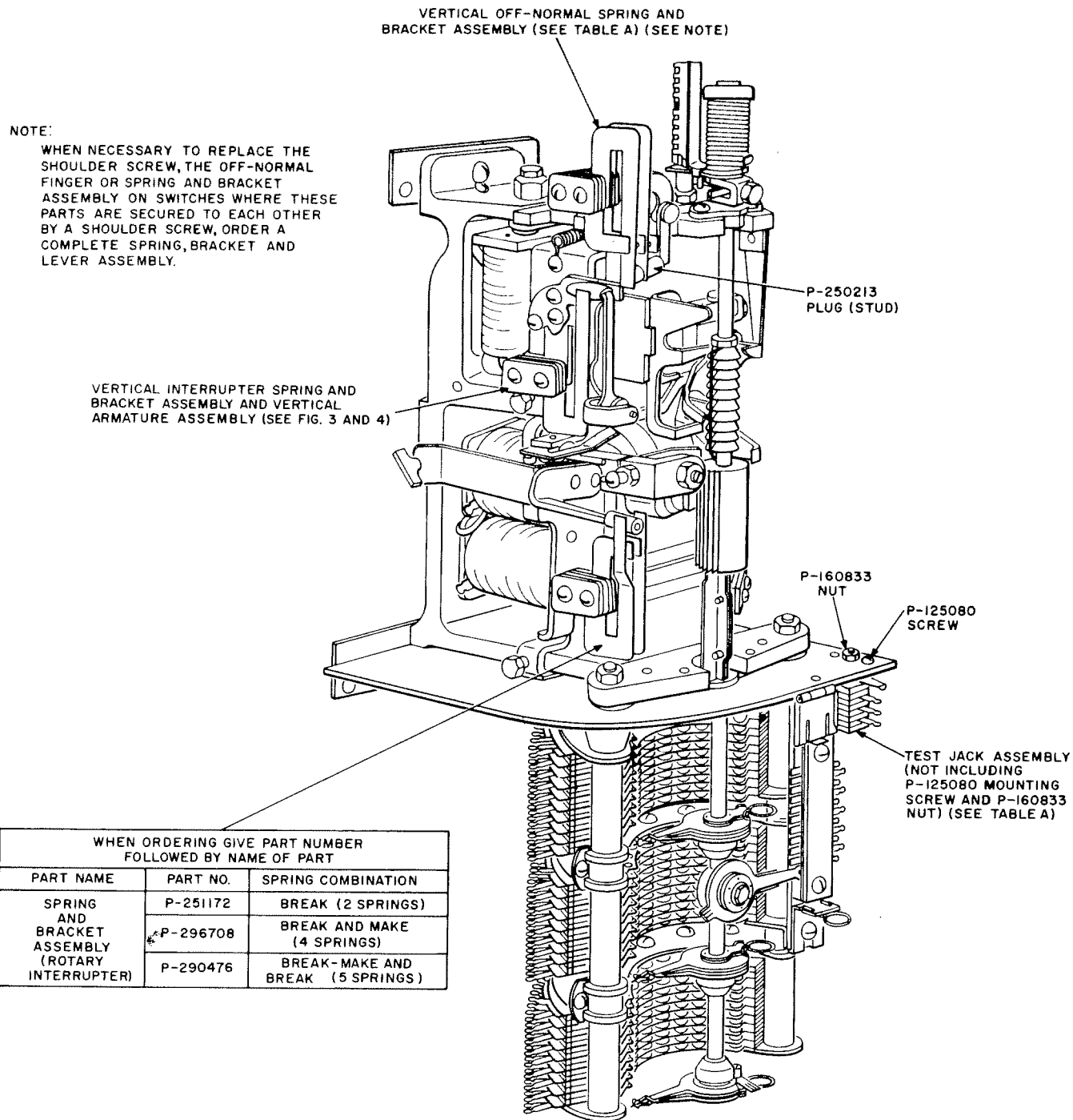
Fig. 1 — Contact Spring Assemblies, Test Jack Assemblies, and Associated Parts of 197-Type Switch as Viewed From the Left Side
