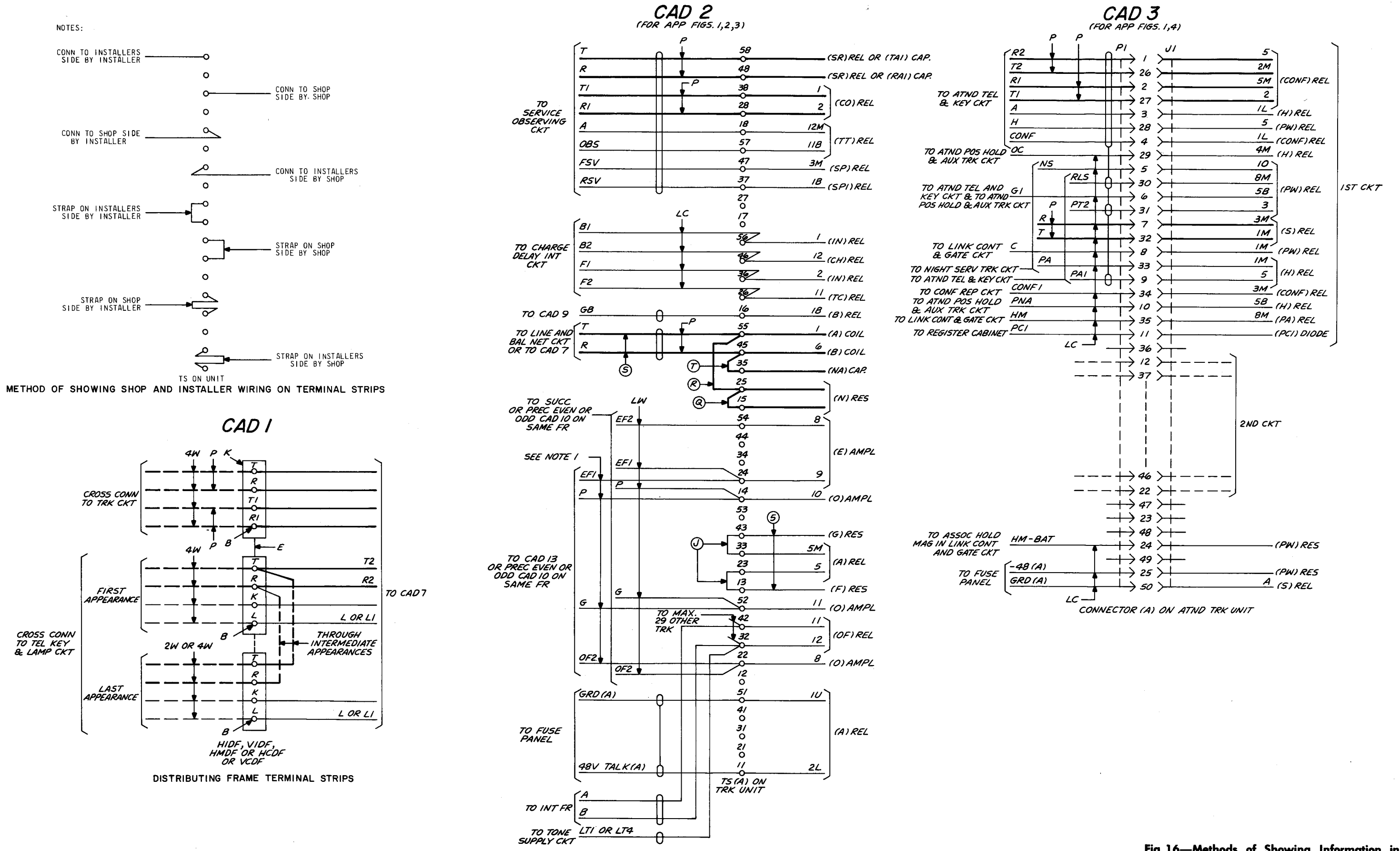
Fig 16—Methods of Showing Information in Cabling Diagrams
