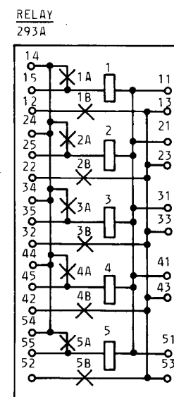
Fig 5F—Alternative Method of Showing Dry Reeds
