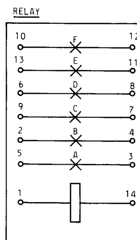
Fig 5H—Alternative Method of Showing Dry Reeds
