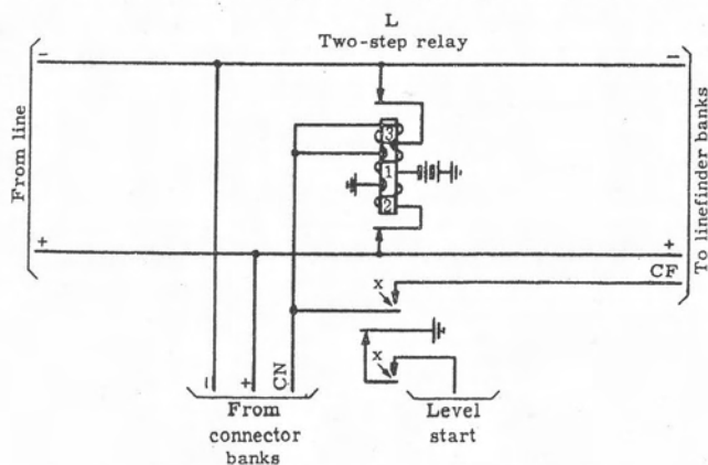
Figure 7. One-relay line circuit, using "2-step" relay.
