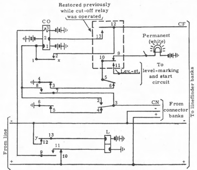
Figure 34. Two-relay mechanical-lockout line circuit.
