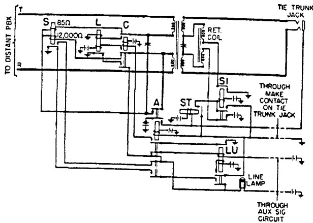
Fig. 17—Automatic Tie Trunk
