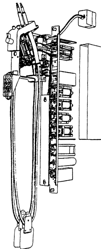
Fig. 3—Cord Circuit Unit
