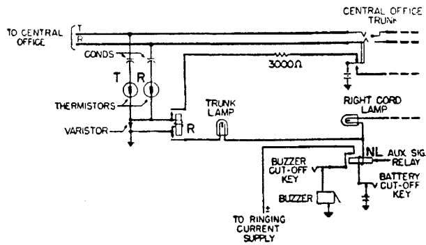
Fig. 15—Central Office Trunk Circuit
