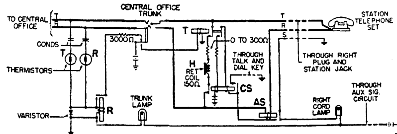
Fig. 8—Through Supervision on All Calls
