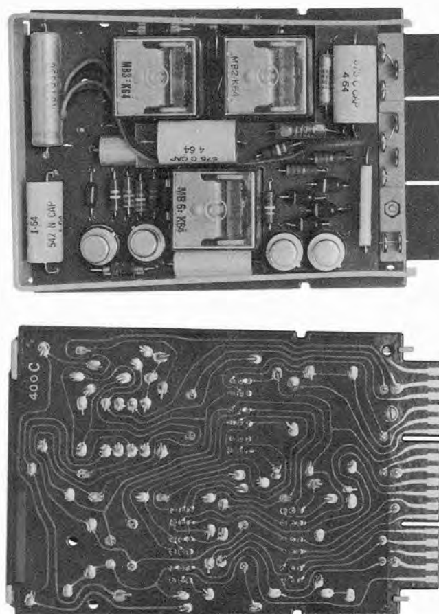
Fig. 2 — 400C Key Telephone Unit
