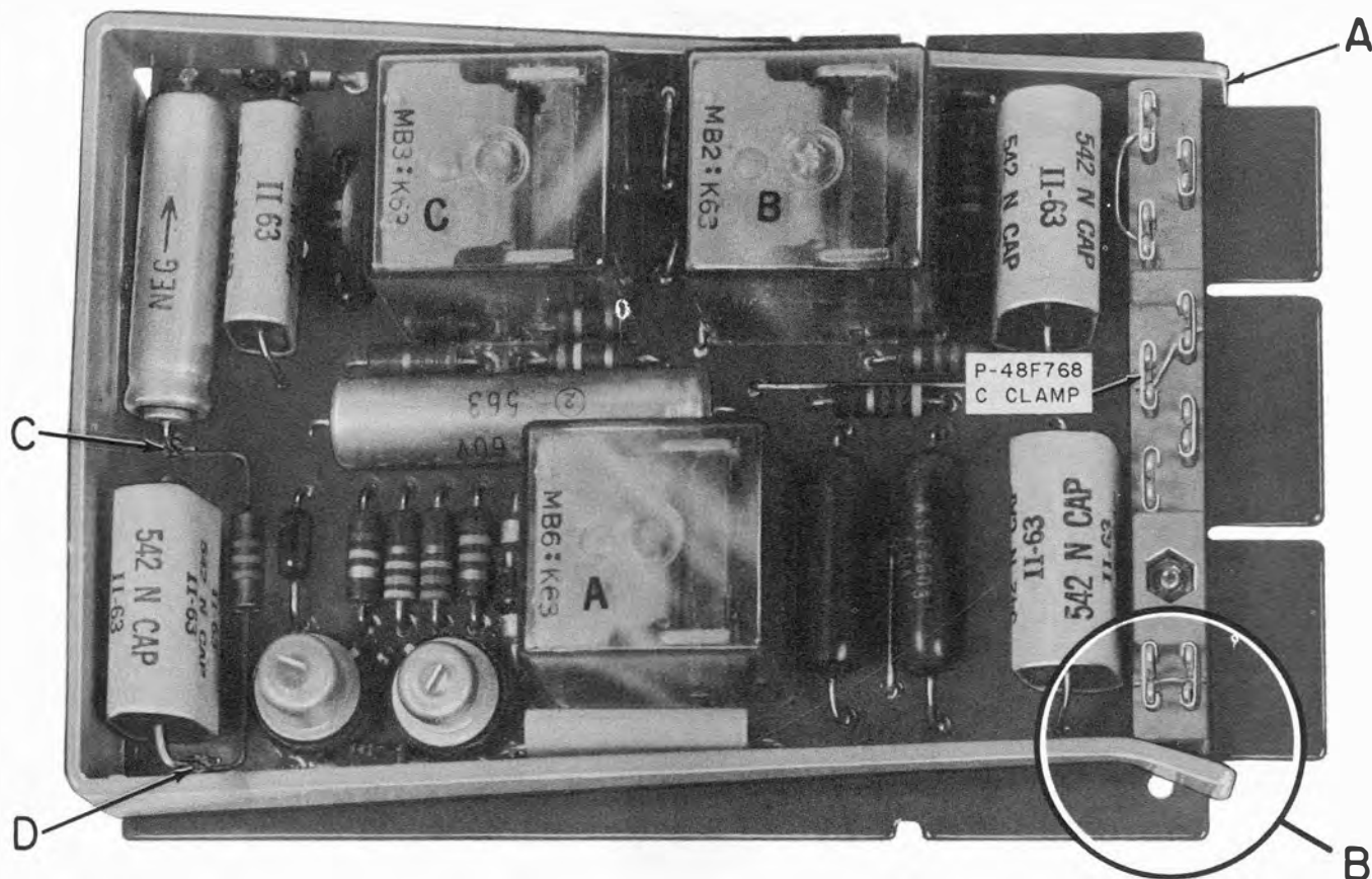
Fig. 4 — Modification of 400B or C KTU
