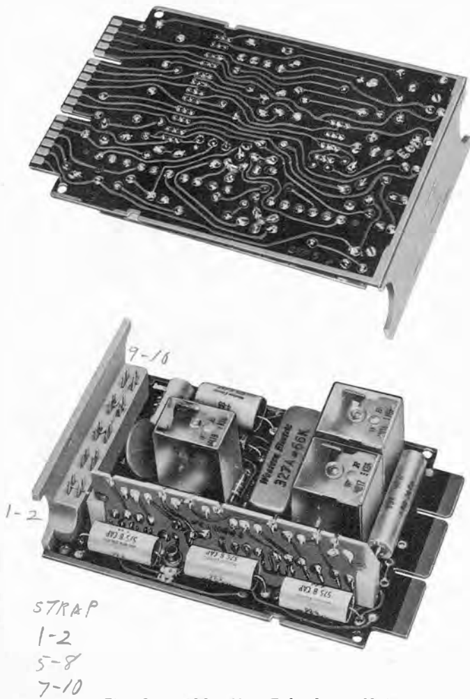
Fig. 3 — 400D Key Telephone Unit
