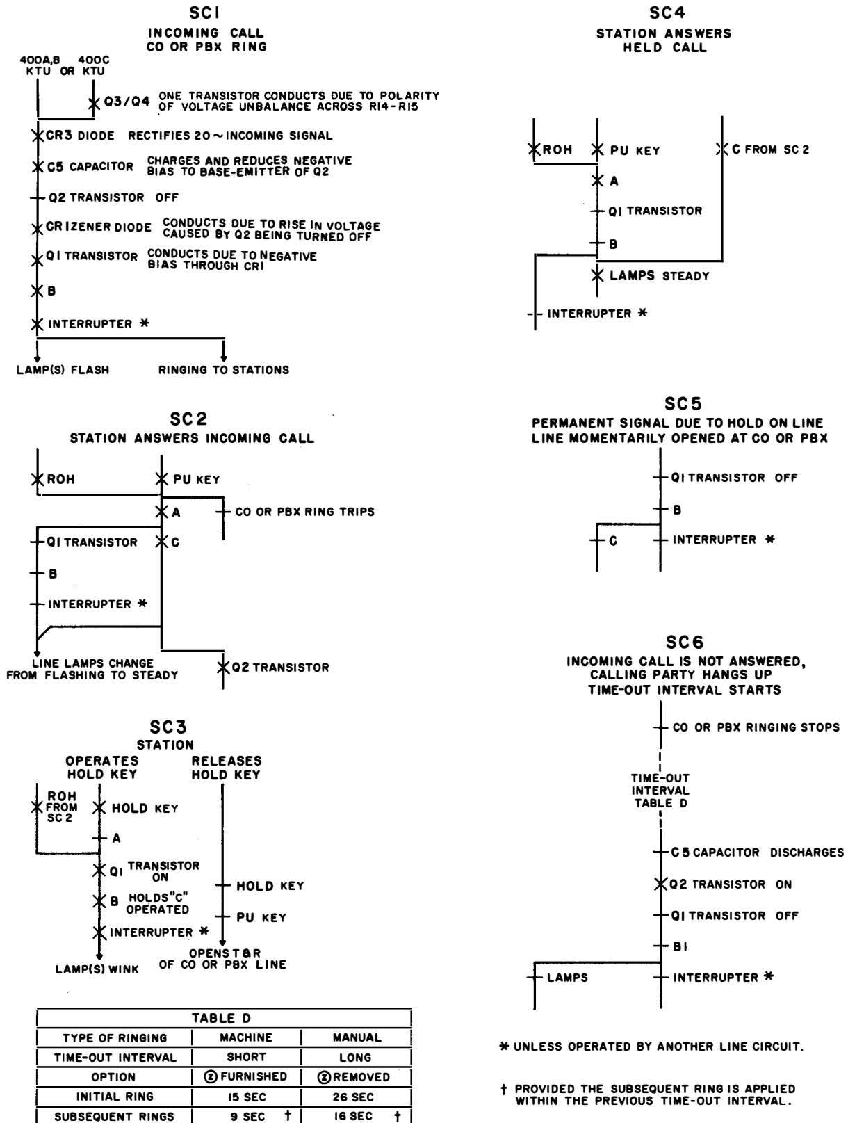
Fig. 7 — Sequence Charts (SC1 to SC6) Showing Operational Sequence of 400A, B, and C KTUs
