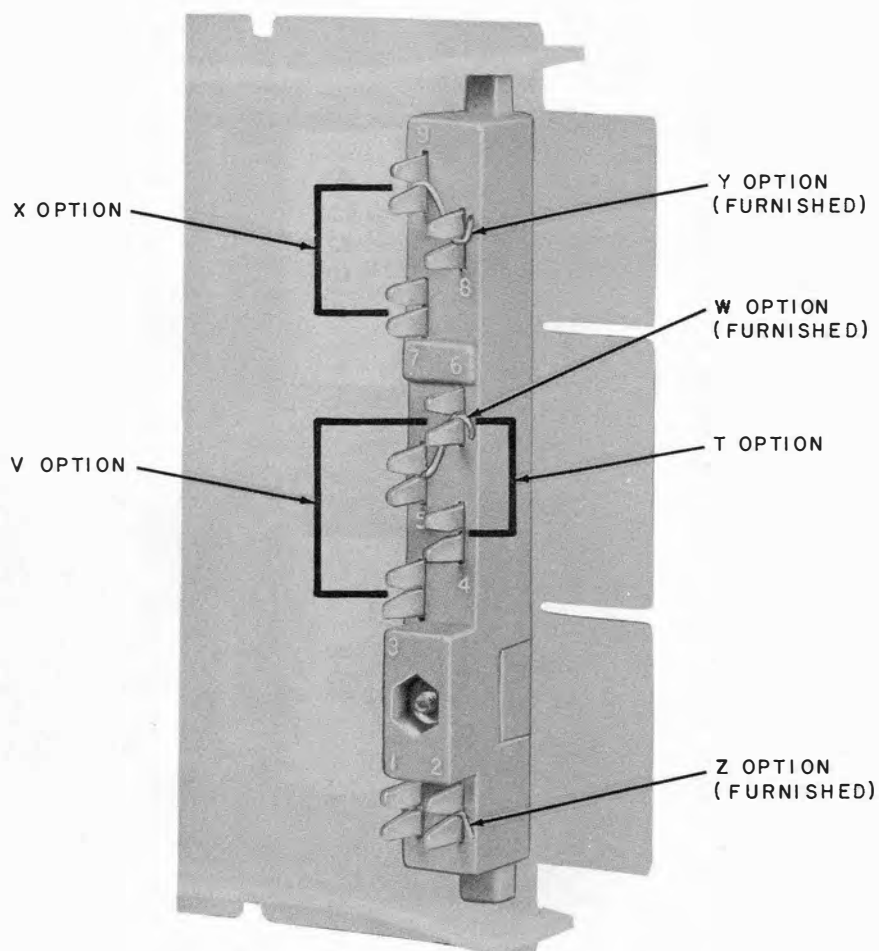
Fig. 5 — Option Block, 400A, B, and C KTUs
